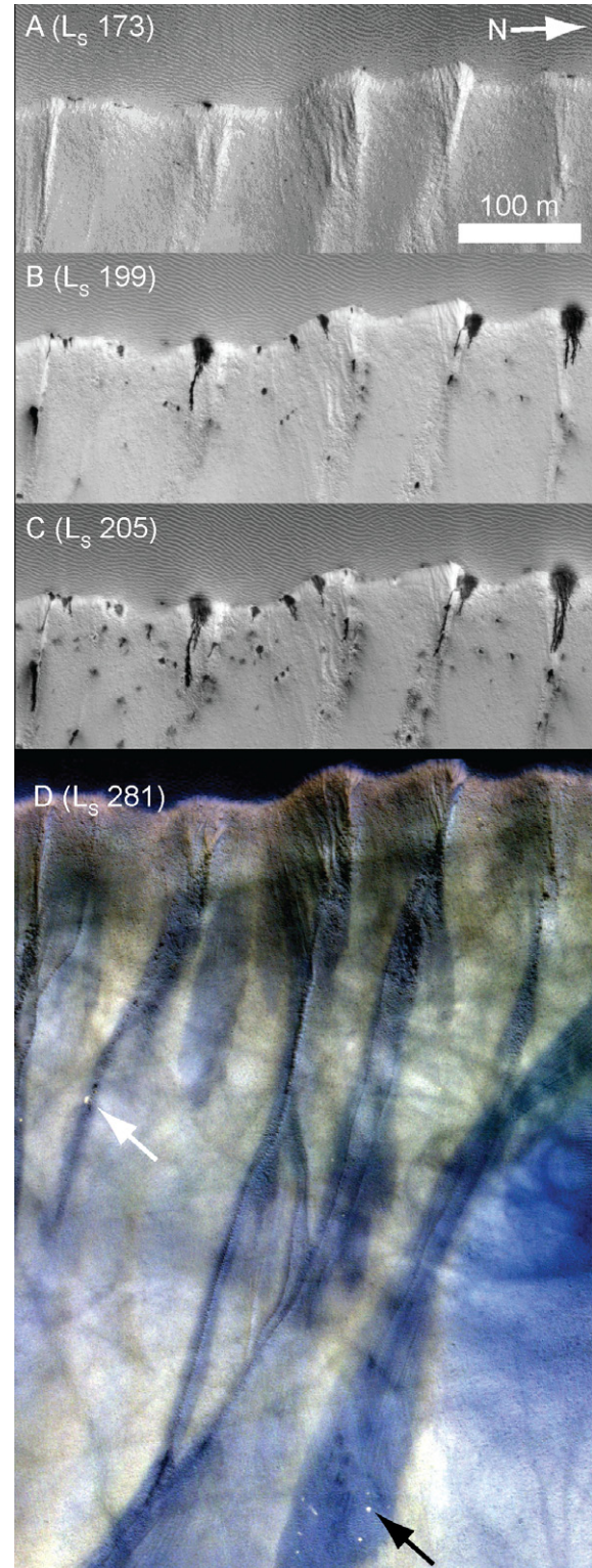
Fig. 6. (A–C) Appearance of dark spots and the associated extension of dark lineae within gully alcoves in dune gullies found within an unnamed crater at 70°S, 178°E (ESP_019987_1095, ESP_020554_1095 and ESP_020699_1095). (D) Is an enhanced-color image of the defrosted surface showing the formation of dark fan-shaped aprons (ESP_022255_1095); these aprons often contain blocks, some of which are bright. Over time, these blocks fade and disappear, suggesting that they are primarily composed of ice. An unstretched image is available in the Supplementary Online Material . All panels are at the same scale.
