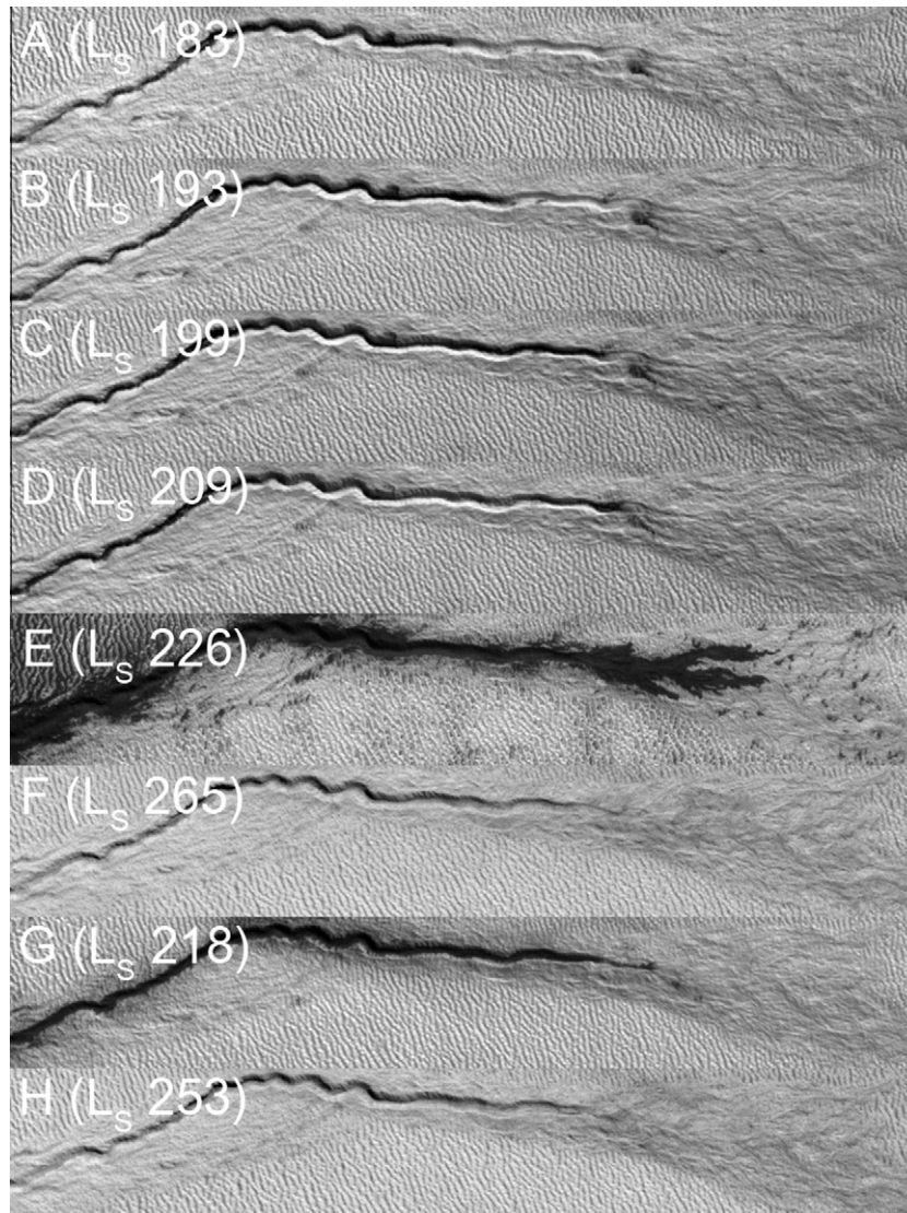
Fig. 11. Another style of activity in a gully channel: advance of a wave of darkening along a frosted channel (A–C), apparent refrosting or disappearance of dark material (D), emplacement of a large dark flow on a surface beginning to defrost (E), and defrosted surface (F). (G and H) The following Mars year: similar channel darkening (G) and defrosted surface (H). Note changes at channel toe when comparing (D–F) and (F–H); extreme albedo contrast makes comparing with E and G difficult. Cutouts are individually stretched for contrast. (Top to bottom: ESP_011396_1115, ESP_011607_1115, ESP_011752_1115, ESP_011963_1115, ESP_012319_1115, ESP_013097_1115, ESP_020956_1115, ESP_021668_1115.)
