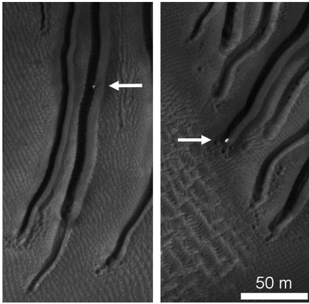
Fig. 5. Ice blocks near channel termini in Russell crater linear gullies (ESP_020784_1255, L_s 209°). The blocks had disappeared by the time these gullies were next imaged, indicating a composition of \text{CO}_2 ice. Note dark haloes around the channels with blocks, suggesting activity within the channel.
