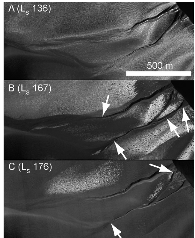
Fig. 3. A new alcove and channel were added to this gully system in Matara crater during MY 30. In addition, substantial changes occurred within the pre-existing gullies, with headward erosion of alcoves, widening and lengthening (and then infilling) of channels, and extension of the debris aprons. From the top, the HiRISE images are ESP_019069_1300, ESP_019636_1300, and ESP_020058_1300.
