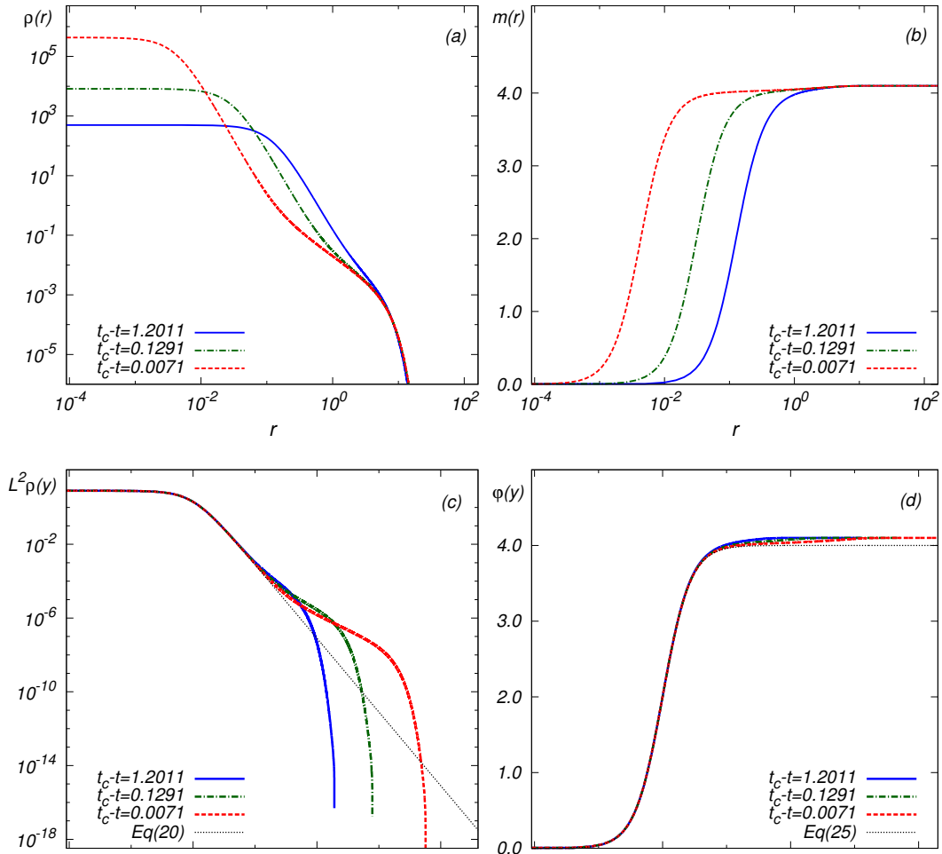
Figure 4.3: The spatial dependence of the density \rho (panels a,c) and the mass m (panels b,d) at different moments of time for the simulation with N = 1.0250N_c . In the top row (panels a,b), the data is shown in simulation coordinates. In the bottom row (panels c,d), rescaled density, L^2\rho(y) , and mass, \varphi(y, \tau) \equiv m(r, t) , are shown as functions of rescaled radius, y = r/L . In panel (a), notice the growth of \rho(r) near the origin and a nearly steady tail. In panel (c), notice the convergence to the static solution (4.11),(4.12) in the growing neighborhood of y = 0 . In loglog scale the deviation from that static solution has the form of a bump. The bump moves away from the origin as t \rightarrow t_c .
