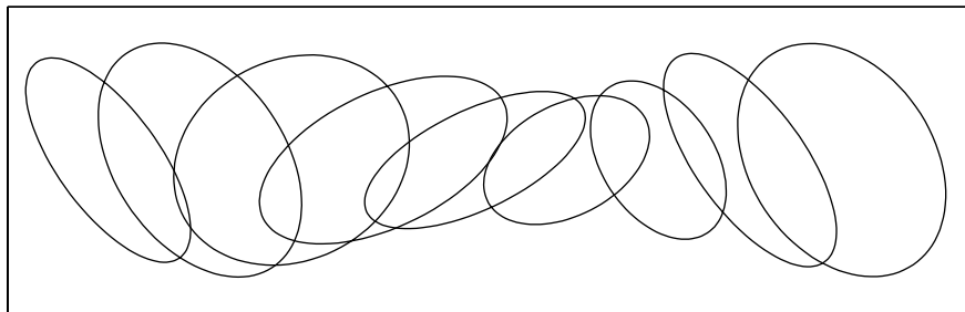
Tumbling: \Lambda=6 , S=10
