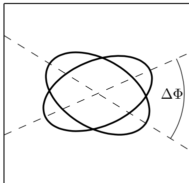
Trembling: \Lambda=1.43 , S=10
