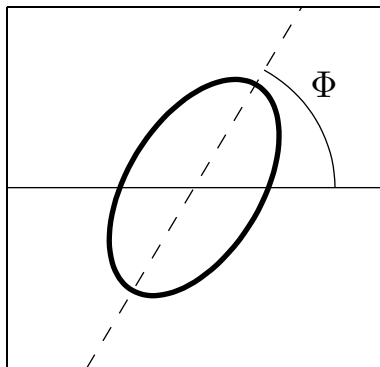
Tank-Treading: \Lambda=0.5 , S=10
