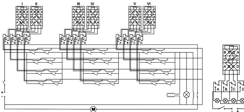
Figure 13. Circuitry of a reduced version of the bomba in comparison with a reduced version of Enigma.
