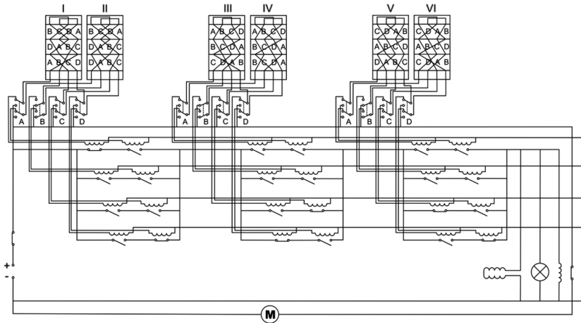
Figure 14. Reduced version of the bomba with current applied.
