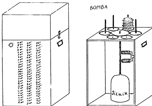
Figure 1. Outside and interior of Polish “bomba”, drawing by Rejewski, 1978 [7, p. 316].
