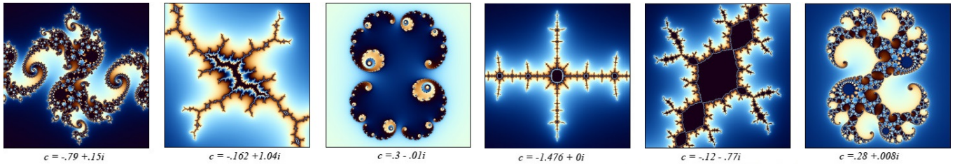
Figure 2: Julia sets for 6 different values of c
