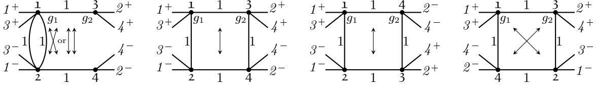
Figure 3: Admissible pairs potentially contributing to (6.4) with d=4
