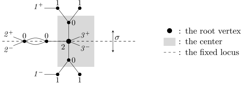
Figure 1: A rooted decorated graph representing an element \mathcal{T} of \mathcal{T}_{7,3}(\mathcal{C})^\phi
