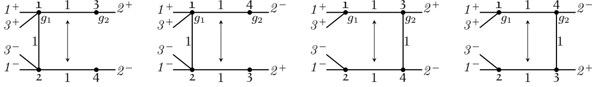
Figure 2: Admissible pairs potentially contributing to (6.4) with d=3
