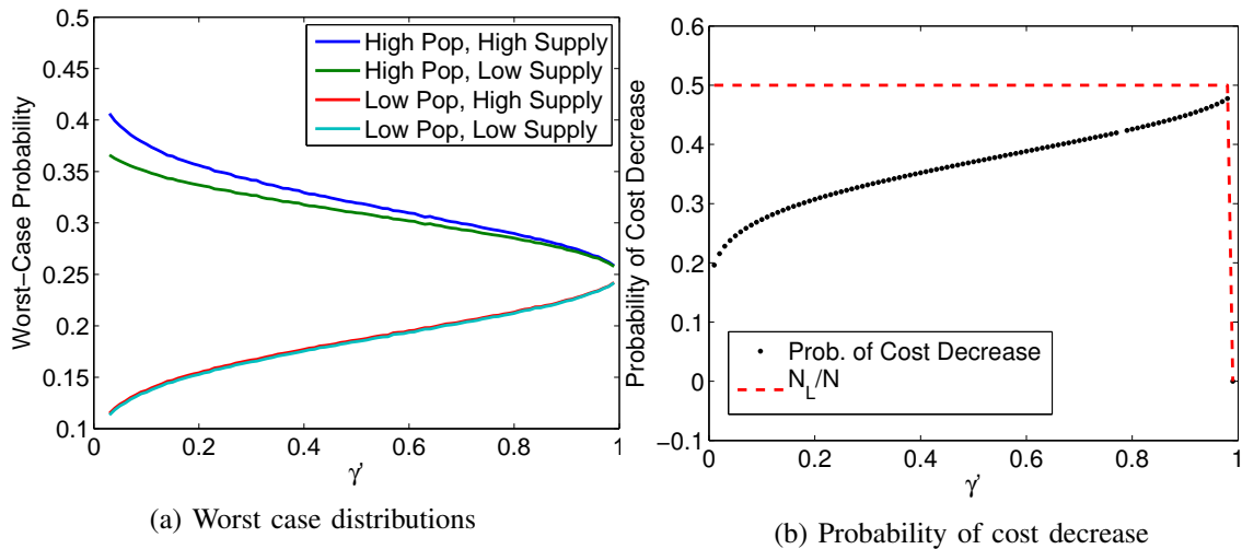
Figure 1: (a) Worst-case distribution for the likelihood robust water allocation problem. (b) Probability that an additional sample causes a decrease in worst-case expected cost for the likelihood robust water allocation problem. The red line shows the upper bound probability \frac{N_L}{N} .
