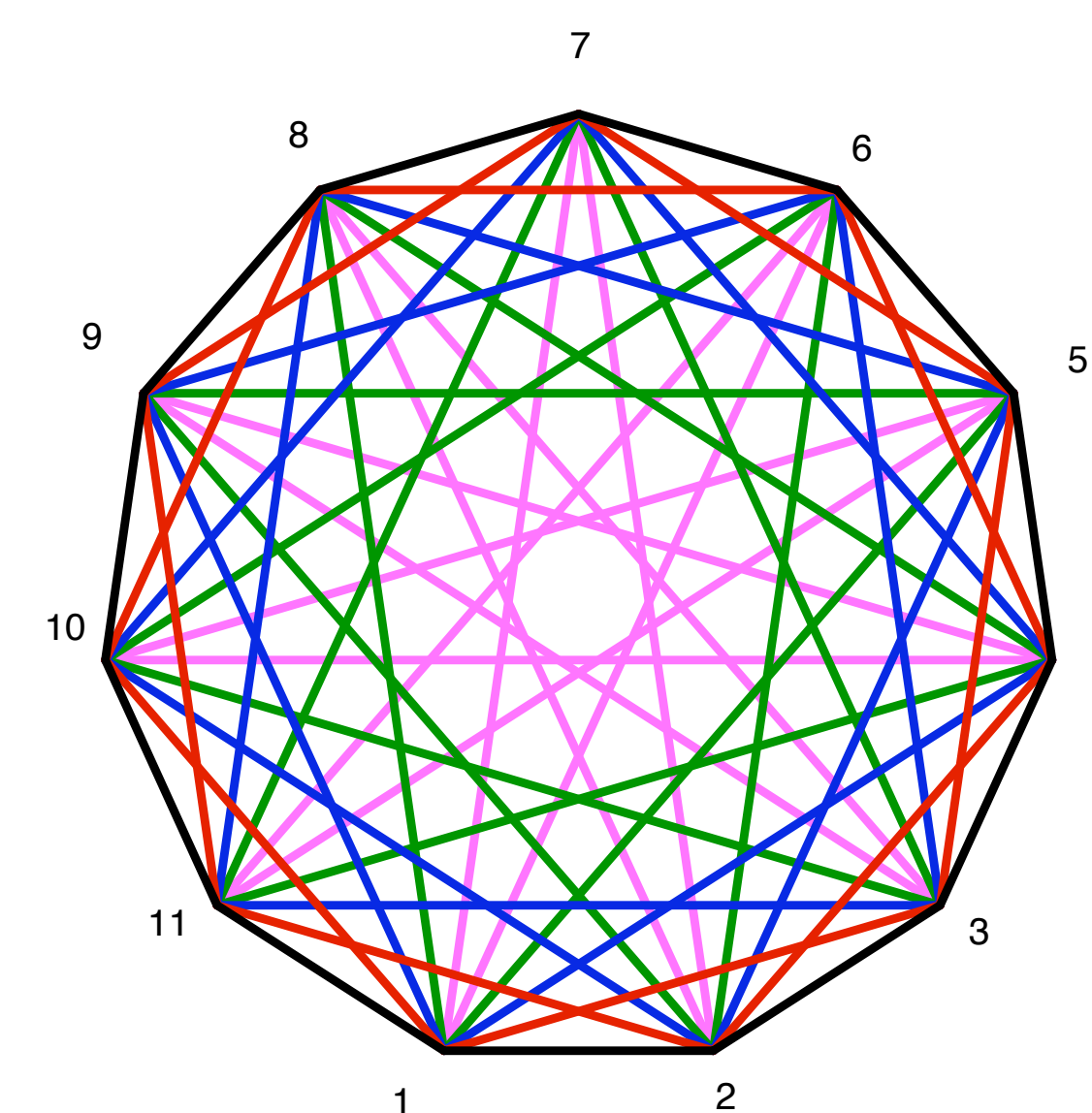
Figure 1: Graph Representation of the boundary of C(11, 4) .
